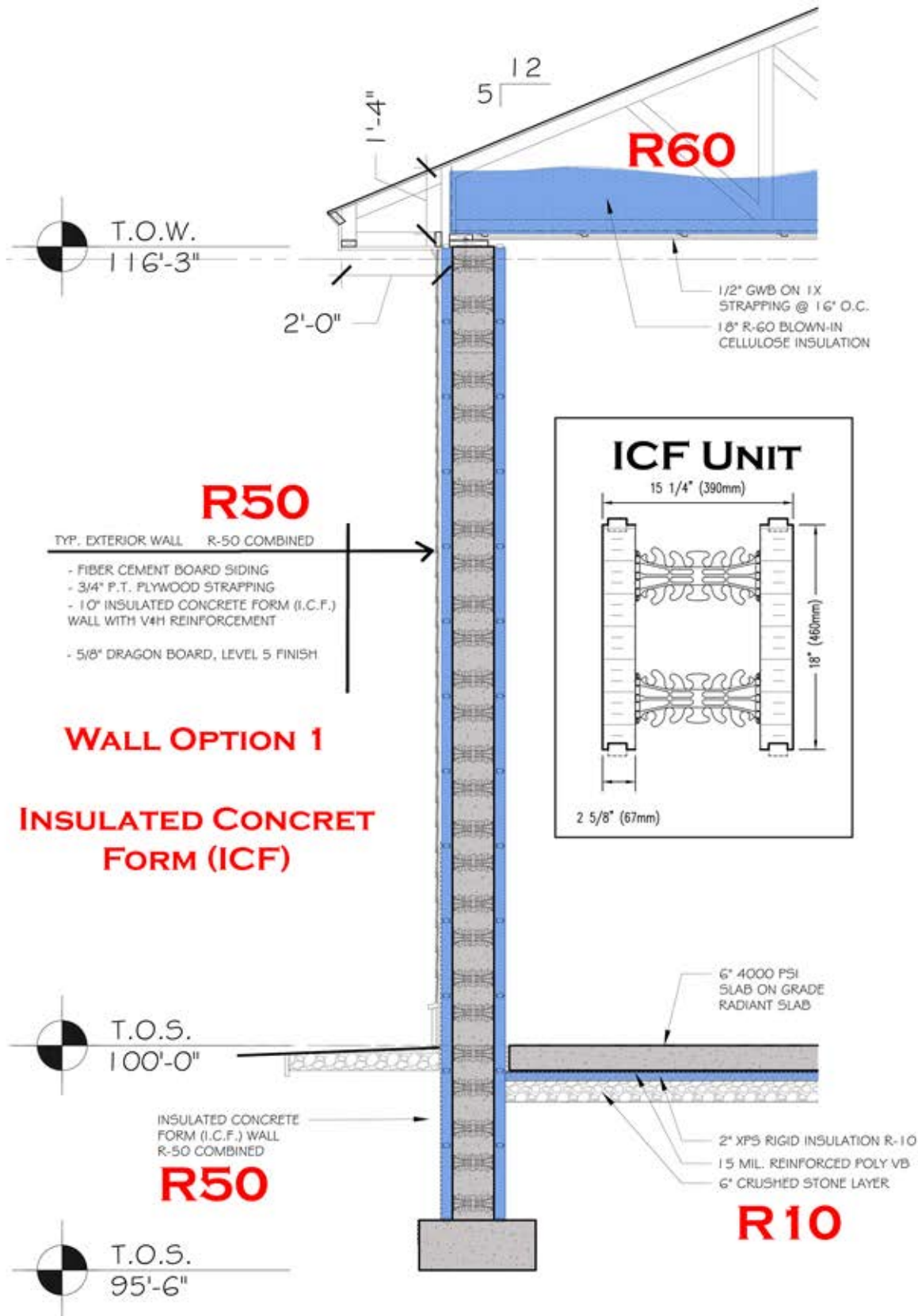
OPTION 1 - INSULATED CONCRETE FORM
