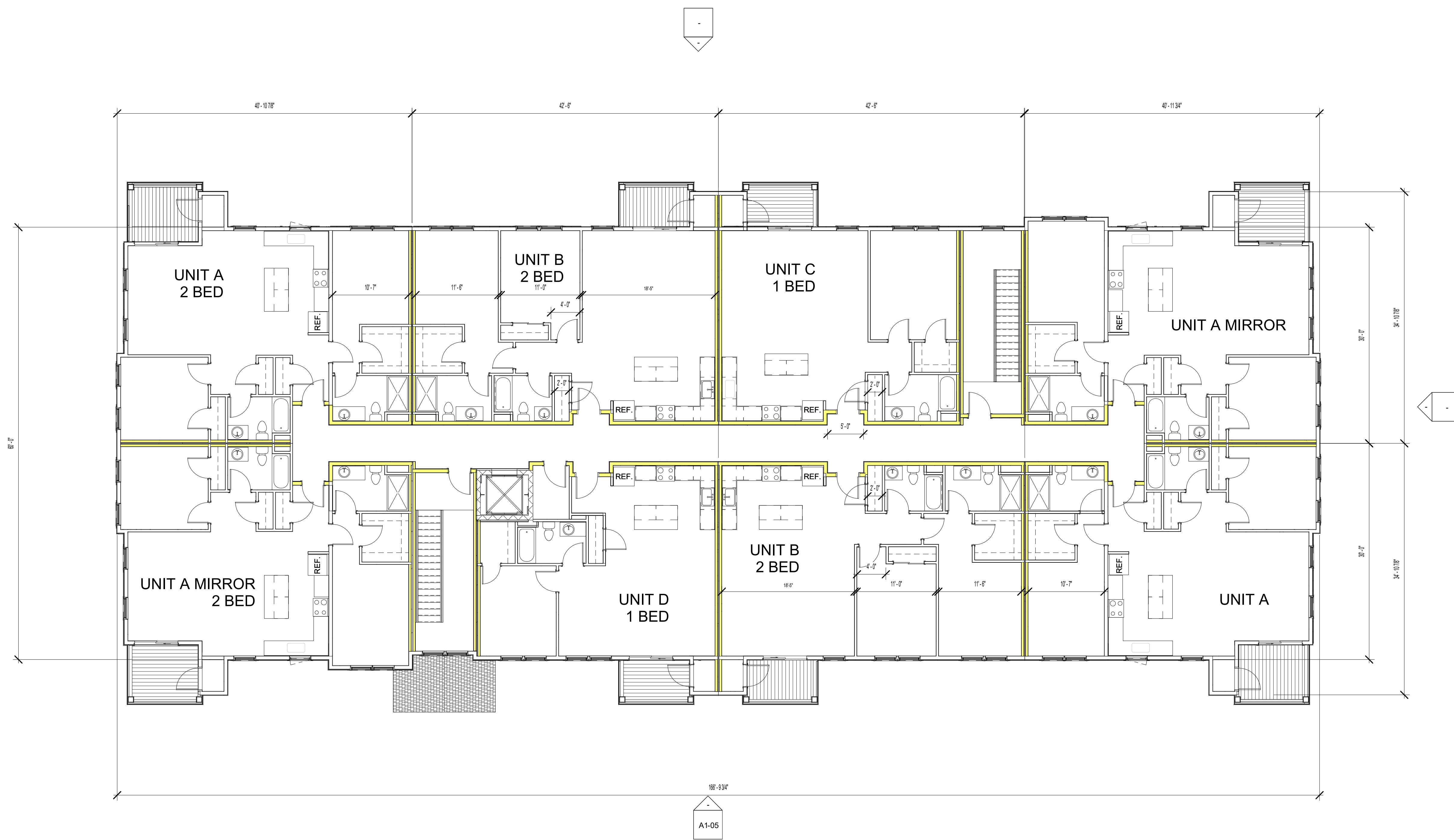
① THIRD FLOOR 1/8" = 1'-0"
